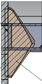
FyreFLEX sealant applied to all gaps, finished with 30x30mm fillet
