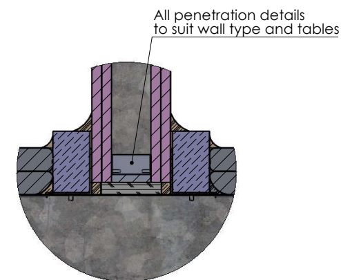
DETAIL i
